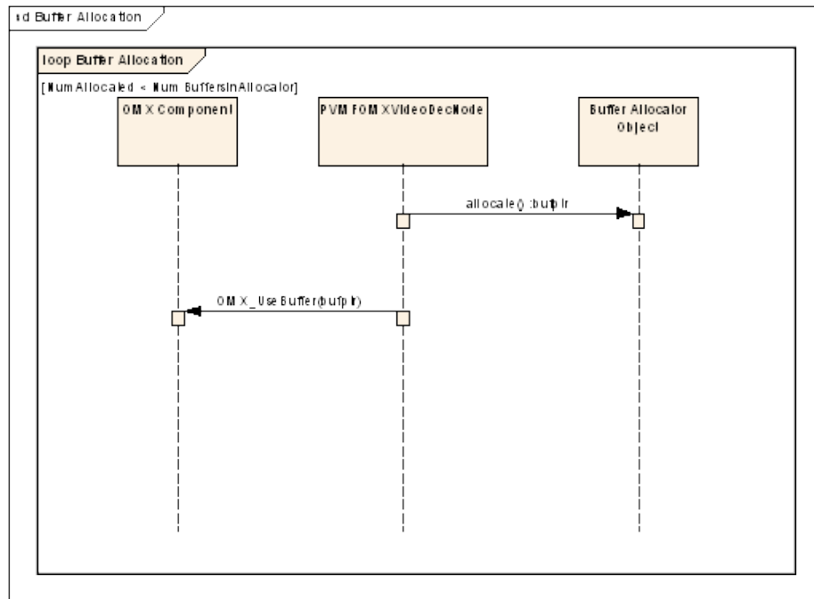
Figure 5: Buffer Allocation
