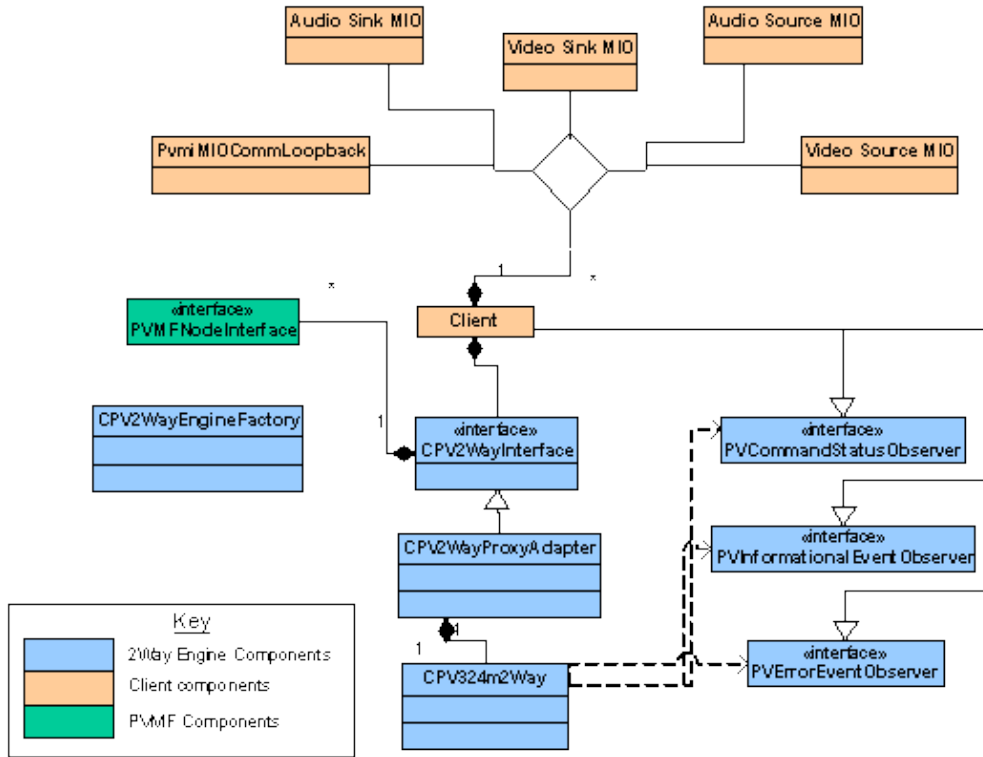
Figure 1: High Level Class Diagram
