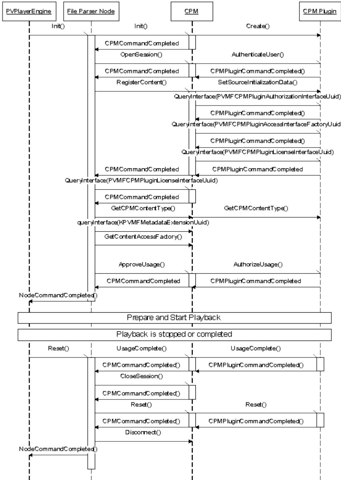
Figure 6: Local Playback of Wrapped DRM Content
