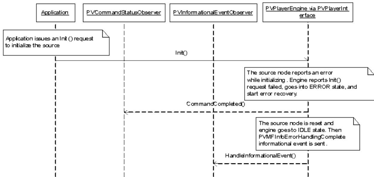
Figure 39: Error Recovery During Initialization
